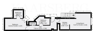
NOT TO SCALE ground floor
